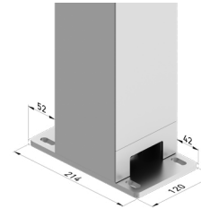
Soporte suelo pilar intermedio Intermediate post floor support
