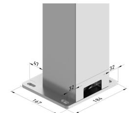
Soporte suelo pilar intermedio a muro Intermediate post floor-to-wall support
